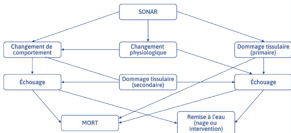
Fig. 4. Potential mechanisms by which cetaceans are affected by sonar (source: authors based on Cox et al., 2006).
