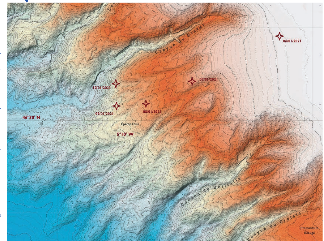
Fig. 5. Reconstruction of the carcass drift (one mark per average daily position) from the stranding site (pink octagon) to the time of death (red capsules, period from January 5 to 10). Vessel presence zone (red circle). Credits: SHOM maps and enlargement on detailed bathymetric survey (Bourillet et al., 2012).
